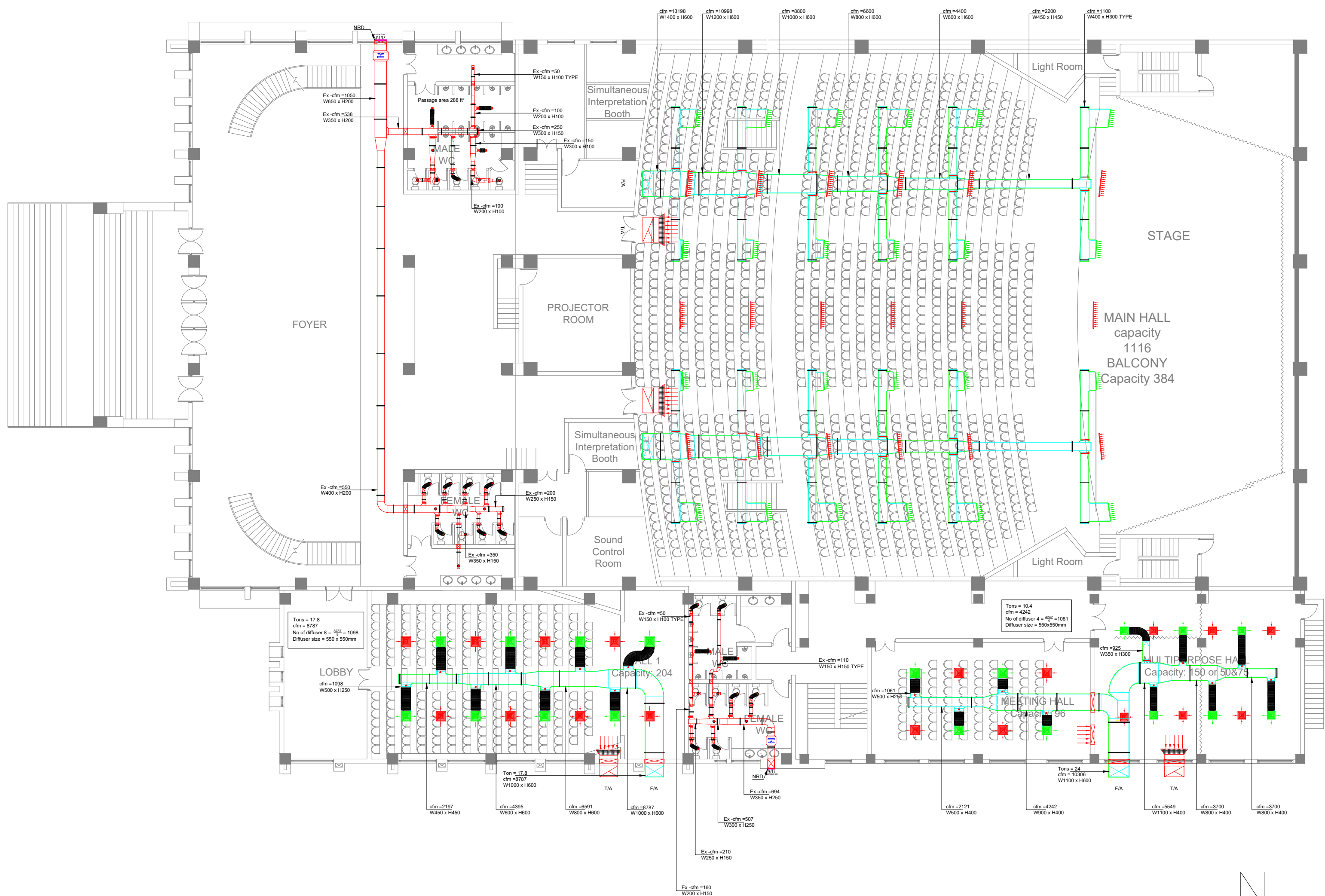
FIRST FLOOR PLAN Area: 2473 Sq.m. Scale= 1:250
